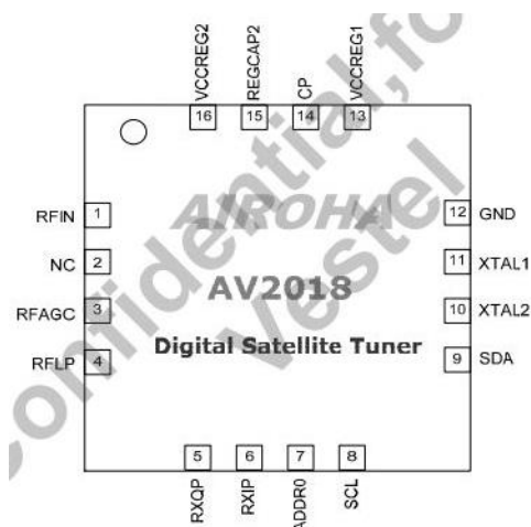
Figure 3: Pin Assignment
